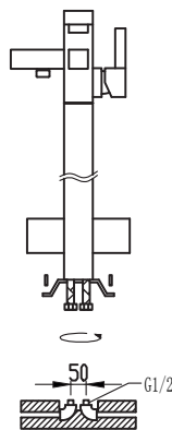
Connect the inlet hose to outlet
